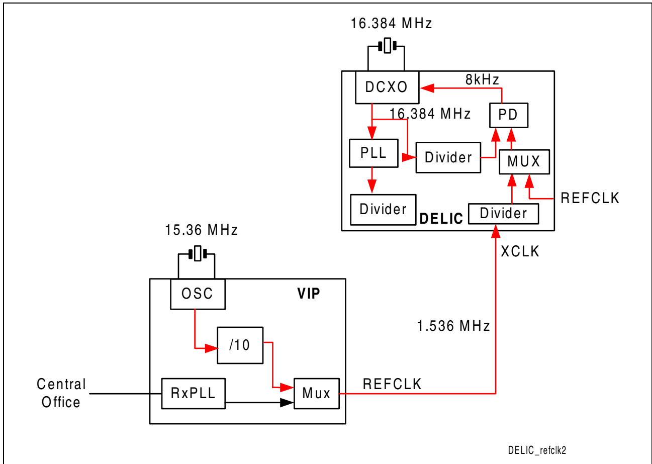
Figure 2 Clocking the VIP by using external Crystal
