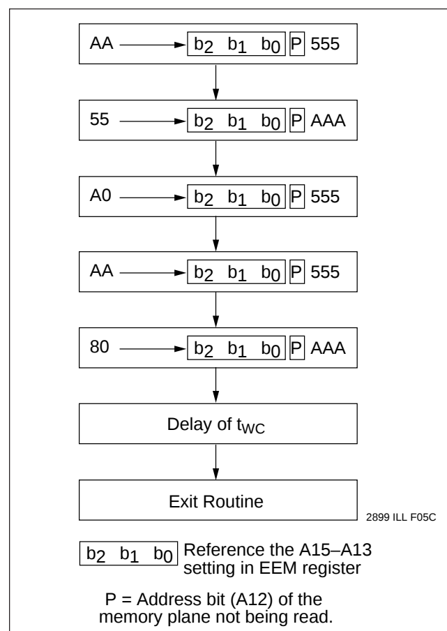
Figure 3. Sequence to Deactivate Software Data Protection
