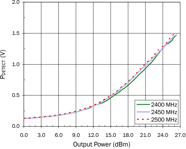
P DETECT versus Output Power over Frequency V cc =3.3V, OFDM 54Mbps, 50% Duty Cycle, Temp=25 °C
