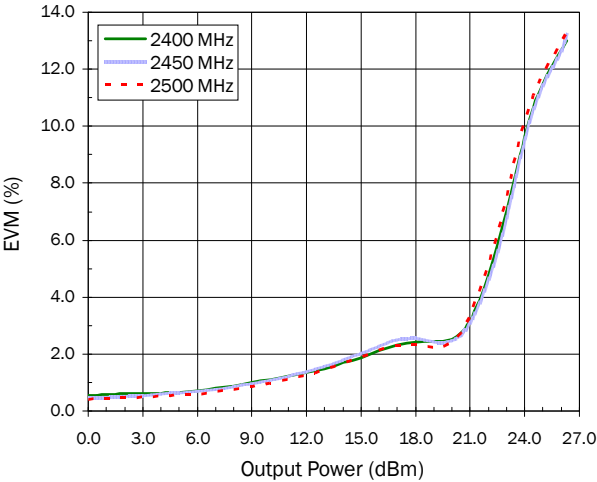
EVM versus Output Power over Frequency V cc =3.3V, OFDM 54Mbps, 50% Duty Cycle, Temp=25 °C
