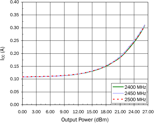
I cc versus Output Power over Frequency V cc =3.3V, OFDM 54Mbps, 50% Duty Cycle, Temp=25 °C
