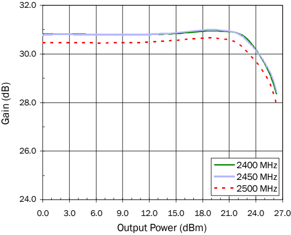
Gain versus Output Power over Frequency V cc =3.3V, OFDM 54Mbps, 50% Duty Cycle, Temp=25 °C
