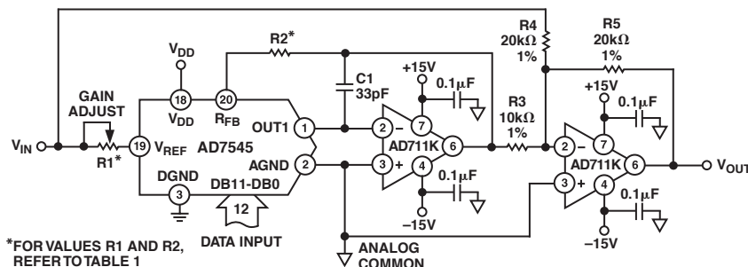
Figure 9. Bipolar Operation
