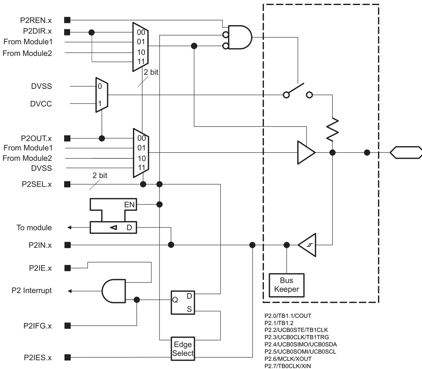
Figure 6-3. Port P2 Input/Output With Schmitt Trigger
