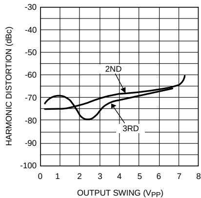
Figure 32. Harmonic Distortion vs. Output Swing (G = +2, V_S = \pm 5\text{ V} , f = 5 MHz)
