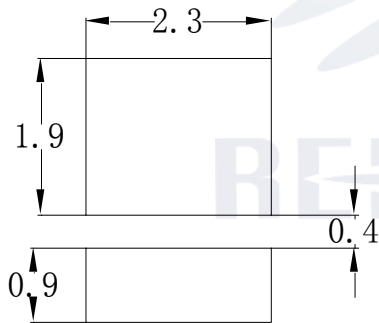
Fig.1-5 Soldering Patterns
