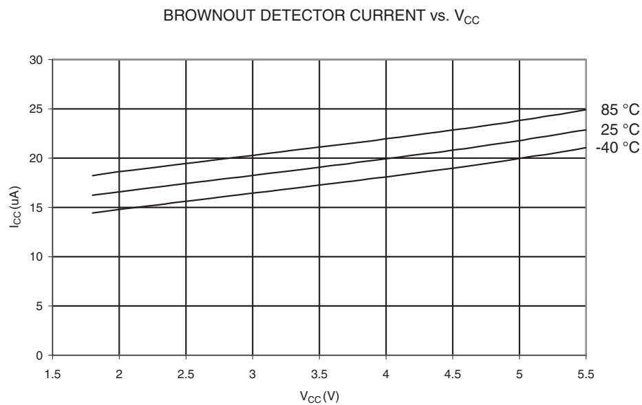
Figure 27-45. Brownout Detector Current vs. V CC
