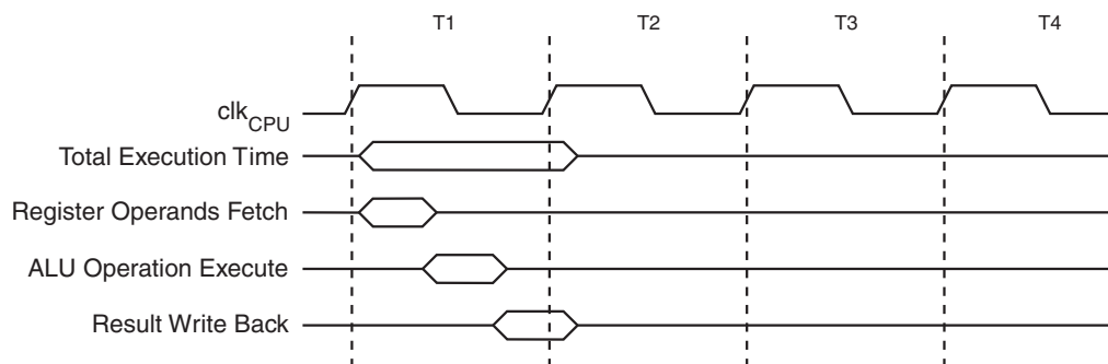
Figure 2. Single Cycle ALU Operation
