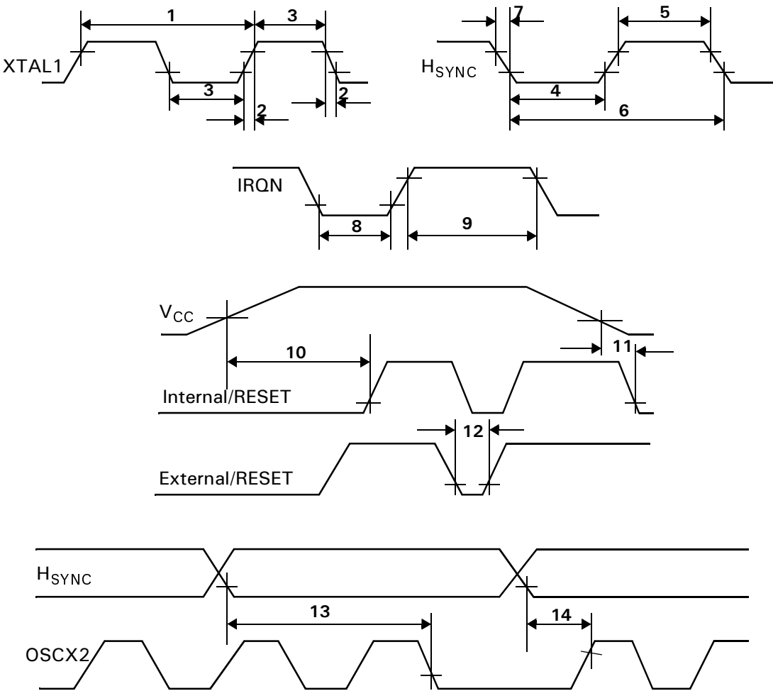
Figure 4. Timing Diagram
