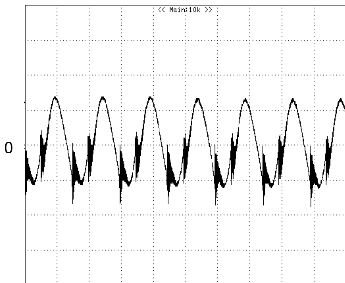
Figure 14: Output voltage ripple at nominal input voltage and rated load current ( I_o=25A ) (10 mV/div, 2 μs/div) Load capacitance: 1 μF ceramic capacitor and 10 μF tantalum capacitor. Bandwidth: 20 MHz. Scope measurements should be made using a BNC cable (length shorter than 20 inches). Position the load between 51 mm to 76 mm (2 inches to 3 inches) from the module
