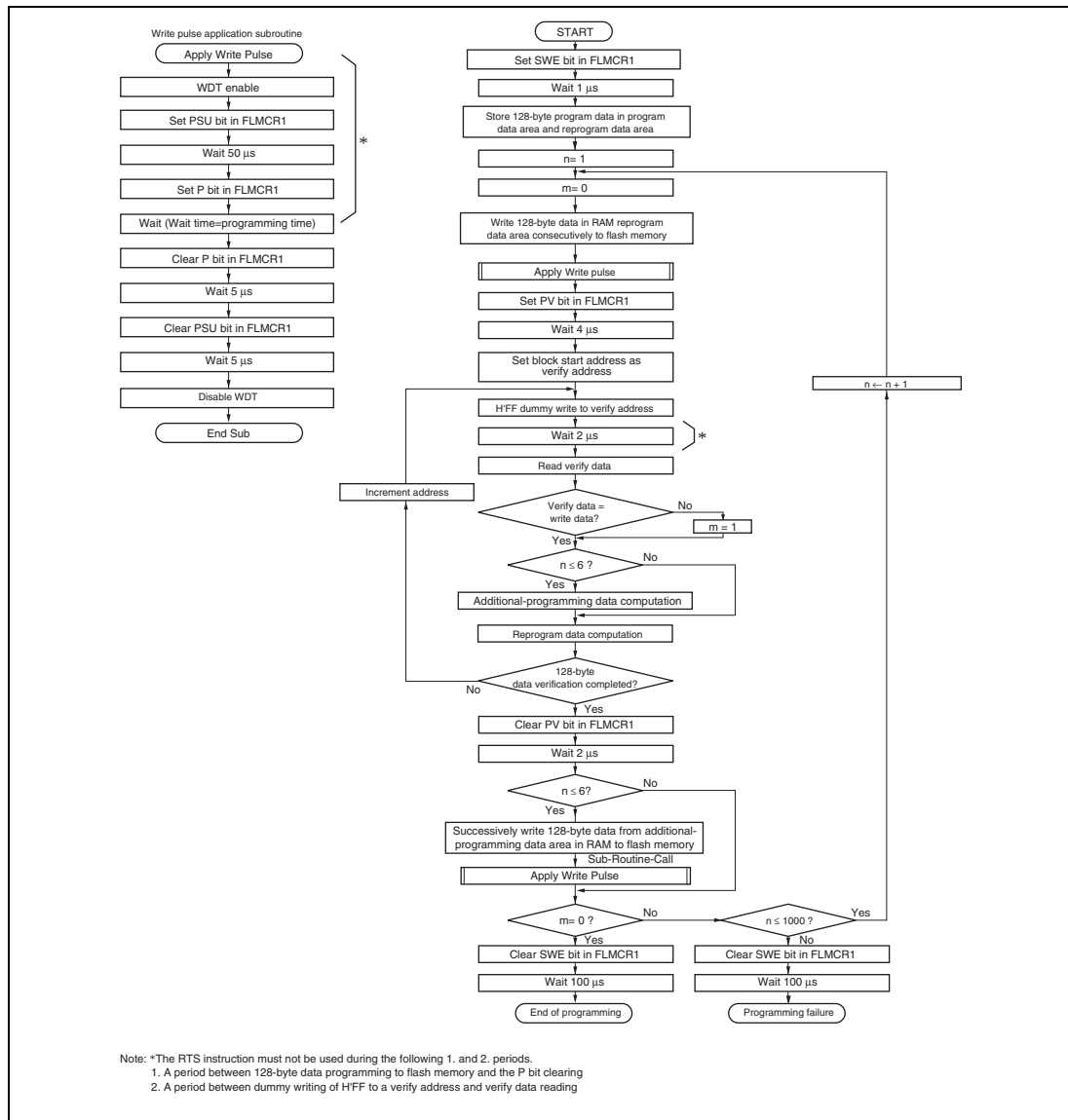
Figure 7.3 Program/Program-Verify Flowchart
