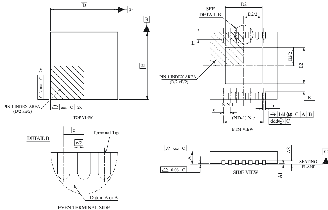
Figure 32. TDFN-8 3x3mm Package
