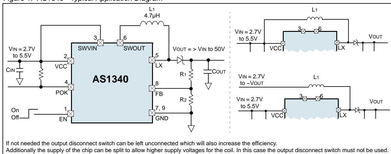
Figure 1. AS1340 - Typical Application Diagram
