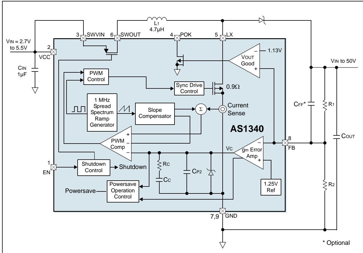
Figure 27. AS1340 - Block Diagram with Shutdown Disconnect Switch
