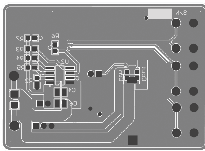
Figure 5: AAT3340 Evaluation Board Rev.1A Solder Side Layout.
