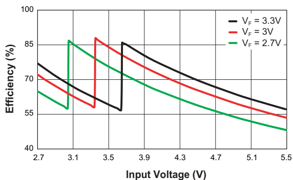
Efficiency vs. Input Voltage (Code 1, BL = 20mA )
