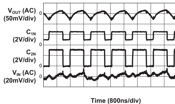
1.5x Mode Load Characteristics ( V_{IN} = 3.3V ; 80mA Load)
