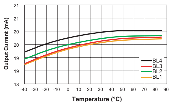
Output Current Matching Over Temperature
