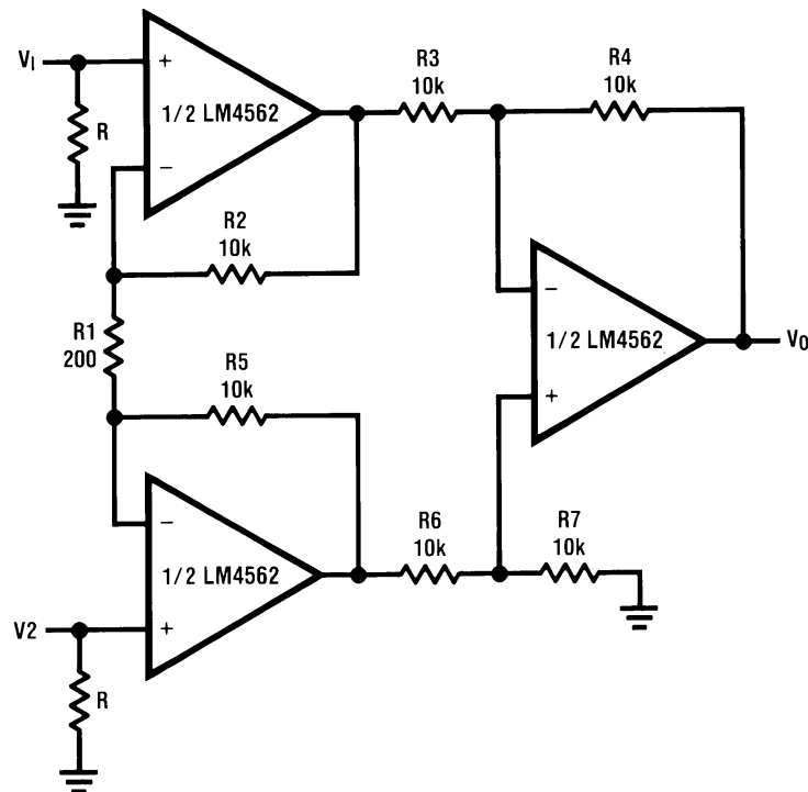
Figure 126. RIAA Preamp
