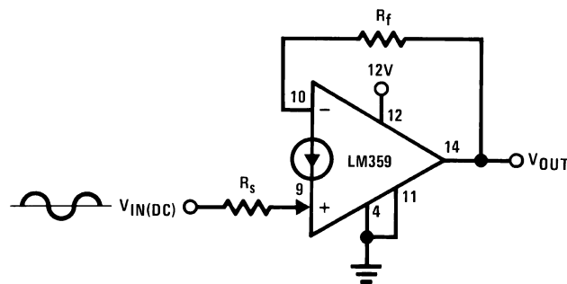
Figure 39. Non-Inverting
