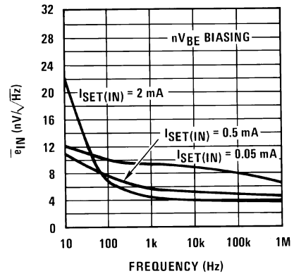
Figure 42. Typical Input Referred Noise Performance
