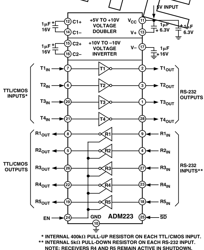
Figure 24. ADM223 Typical Operating Circuit
