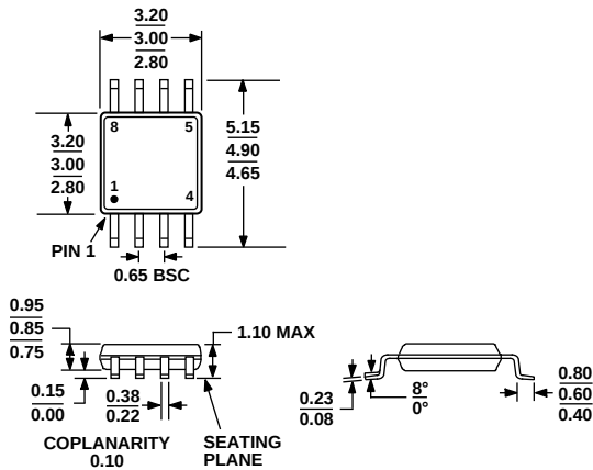
COMPLIANT TO JEDEC STANDARDS MO-187-AA
