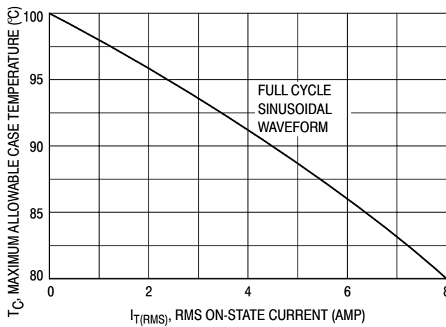
Figure 1. Current Derating
