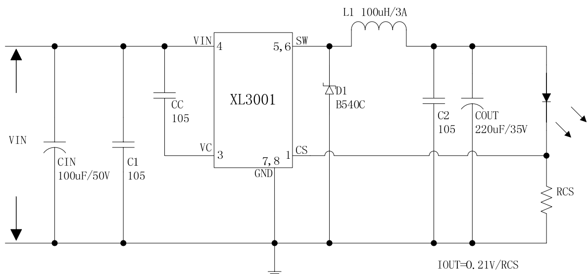
Figure4. XL3001 Typical Application Circuit
