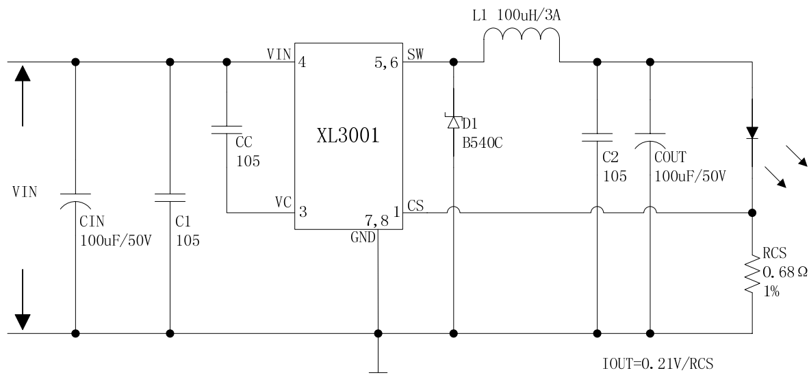
Figure12. XL3001 System Parameters Test Circuit ( V_{IN}=8V\sim40V , I_{OUT}=308mA )
