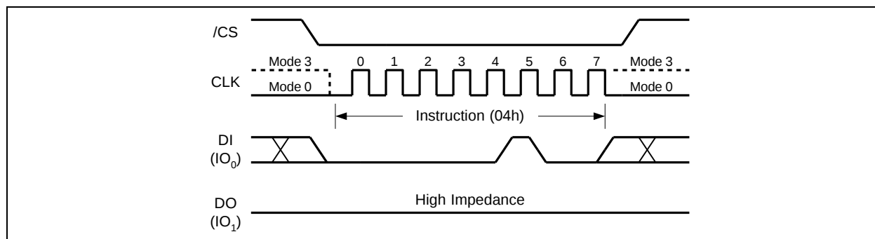
8.2.4 Read Status Register-1 (05h), Status Register-2 (35h) & Status Register-3 (15h)
