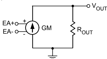
Figure 6. OTA Topology
