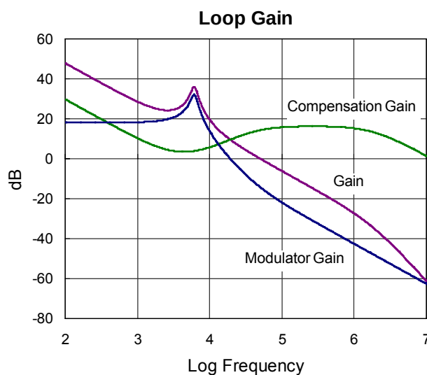
Figure 11. Type 3 Bode Plot
