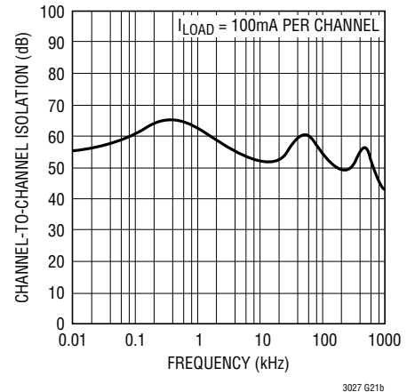
Channel-to-Channel Isolation
