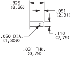
05 .110" QUICK CONNECT
