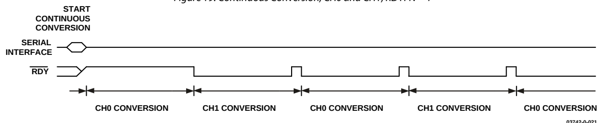
Figure 20. Continuous Conversion, CH0 and CH1, No Data Read
