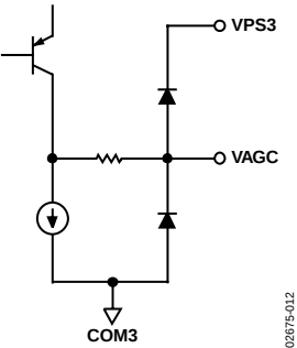
Figure 44. Circuit I
