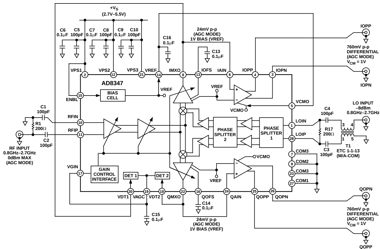
Figure 46. Basic Connections
