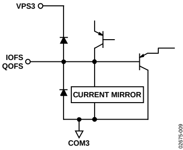
Figure 41. Circuit F
