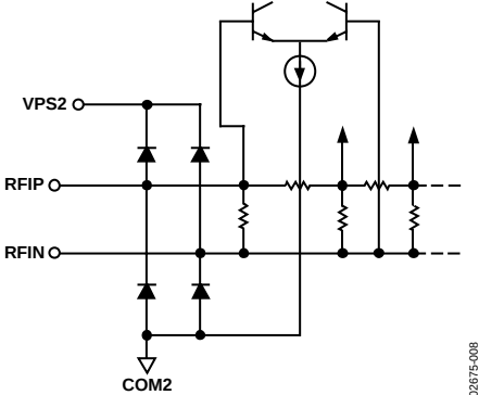
Figure 40. Circuit E
