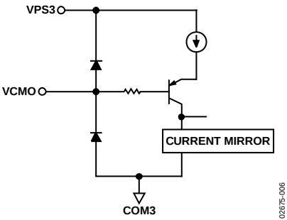
Figure 38. Circuit C
