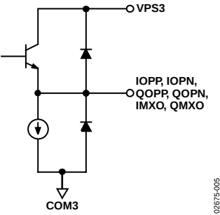
Figure 37. Circuit B
