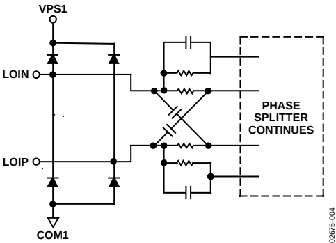
Figure 36. Circuit A
