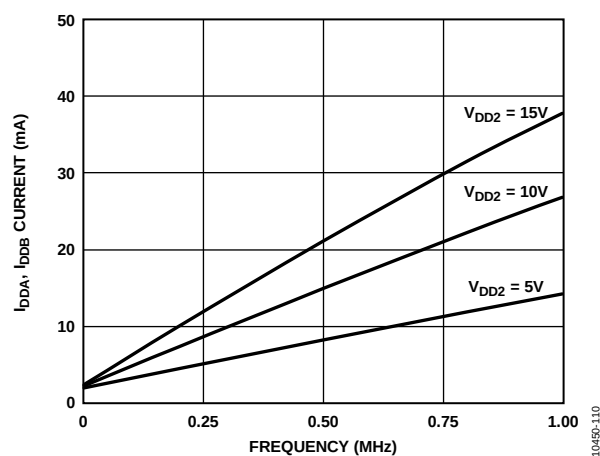
Figure 10. Typical I_{DDA} , I_{DDB} Supply Current vs. Frequency with 2 nF Load
