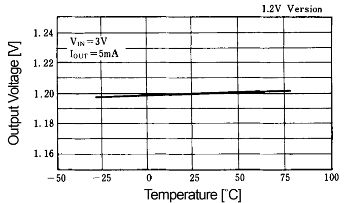
Output Voltage vs. Input Temperature
