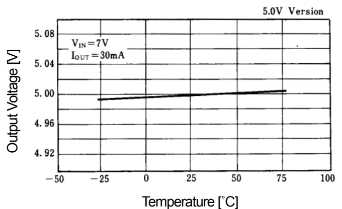
Output Voltage vs. Input Temperature
