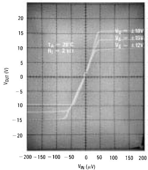
Voltage Transfer Characteristic
