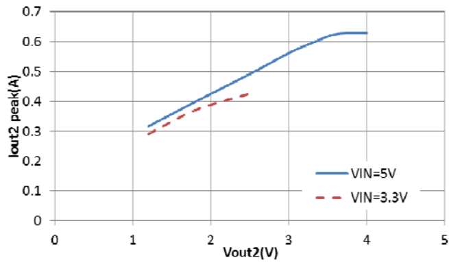
Ch2(LDO) peak output current vs. output voltage (VIN=5.0V)
