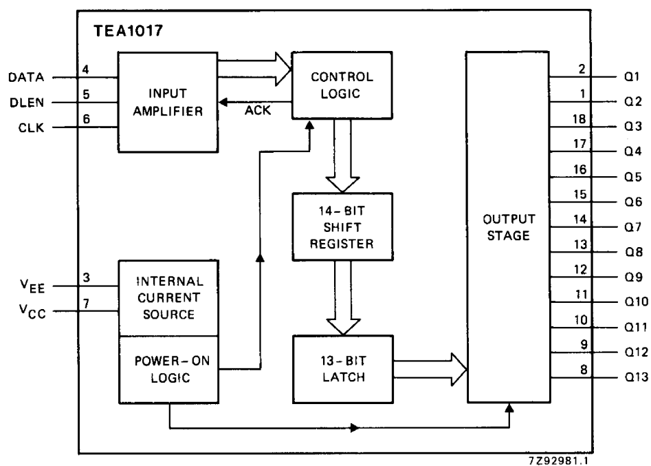
Fig. 1 Block diagram.
