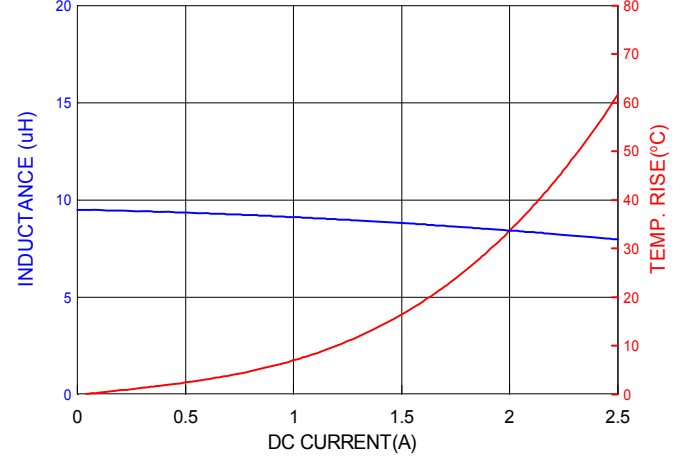
PIT07012-100M
