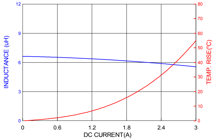
PIT07012-6R8M
