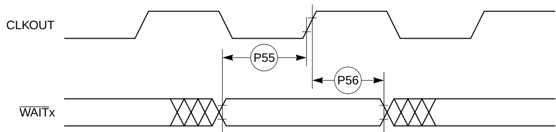
Figure 9-26. PCMCIA \overline{\text{WAIT}} Signals Detection Timing
