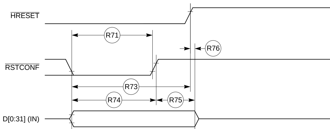
Figure 9-31. Reset Timing—Configuration from Data Bus
