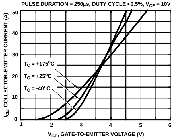
FIGURE 1. TRANSFER CHARACTERISTICS
