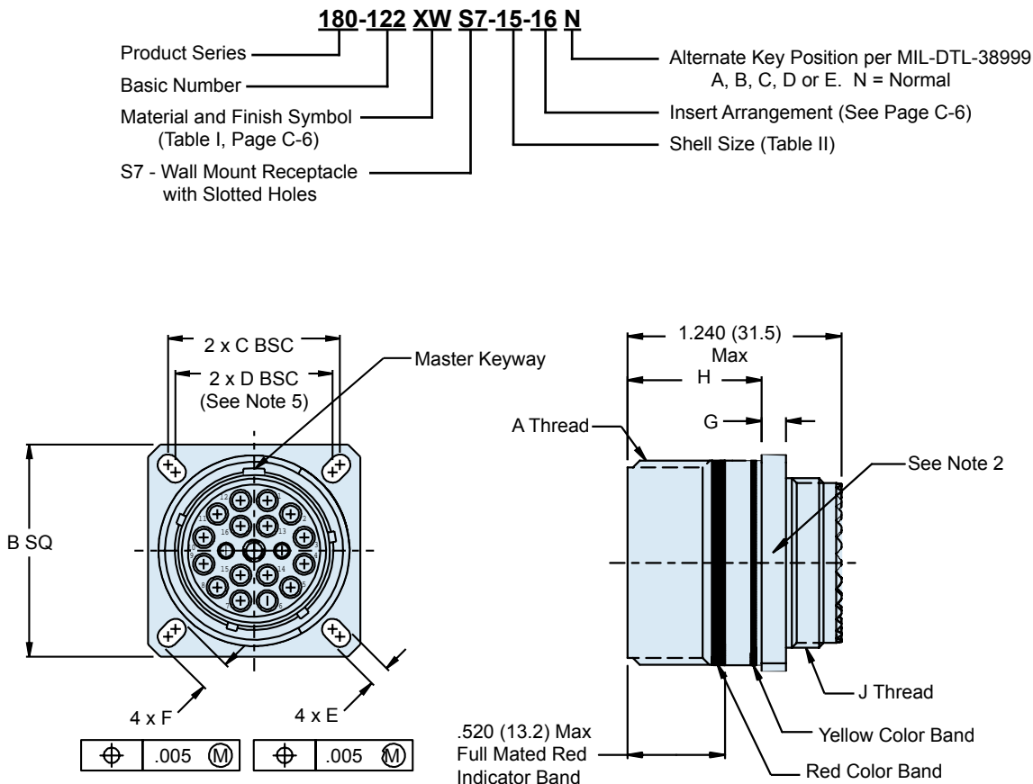
S7 - WALL MOUNT RECEPTACLE WITH SLOTTED HOLES
