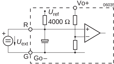
Fig. 9 Voltage adjustment with U_{\text{ext}} between R and Go-
