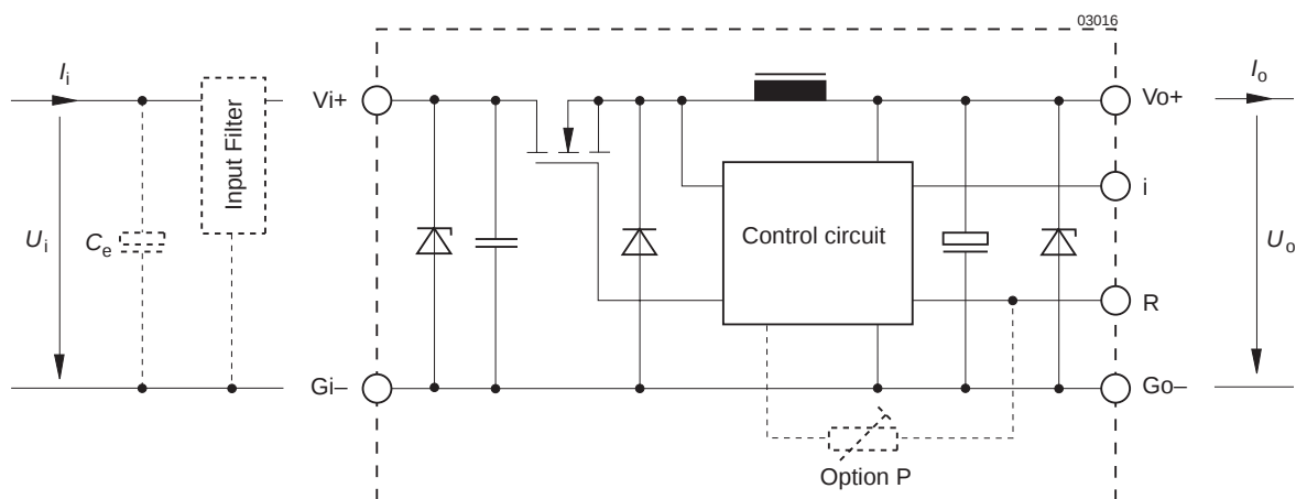
Fig. 1 Block diagram
