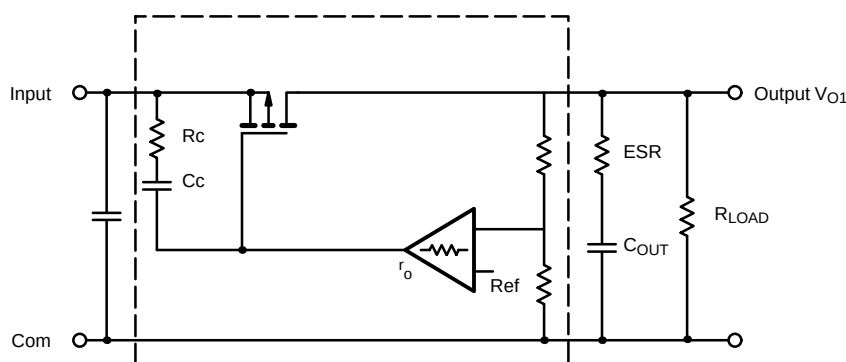
FIGURE 3. Loop Compensation
