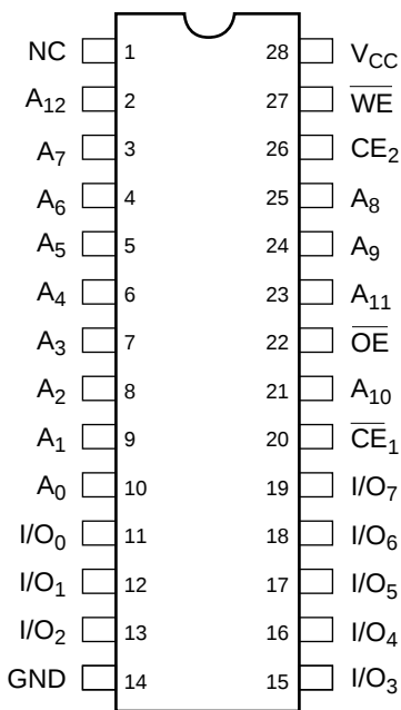
28-Pin SOP
