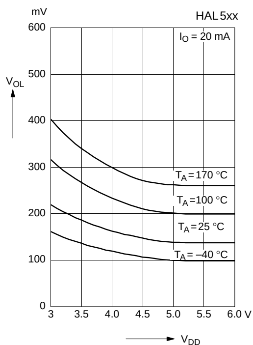
Fig. 3-11: Typical output low voltage versus supply voltage
