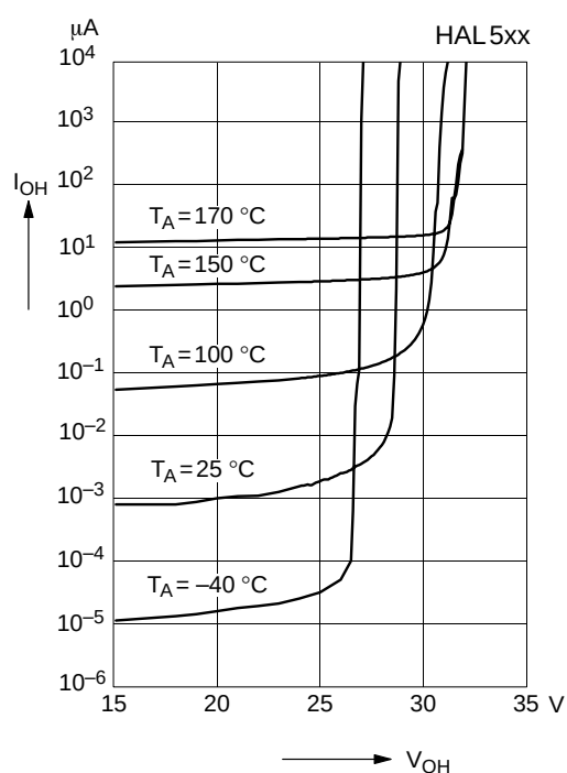
Fig. 3-13: Typical output high current versus output voltage
