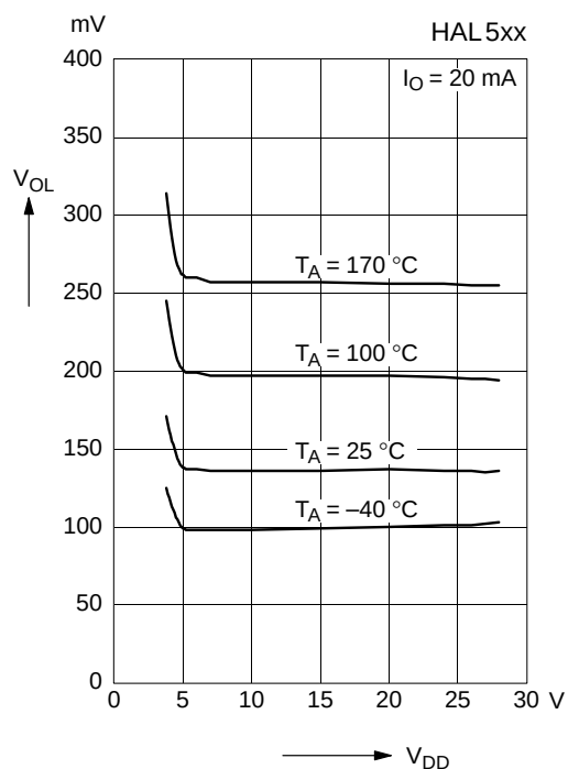
Fig. 3-10: Typical output low voltage versus supply voltage
