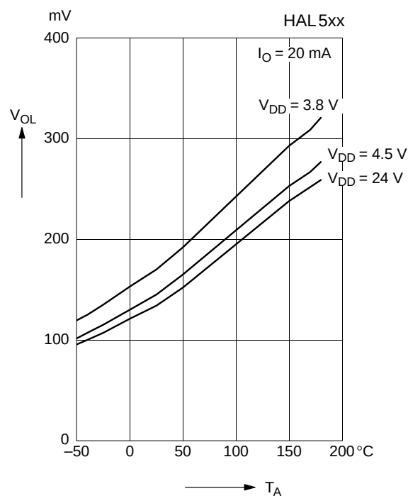
Fig. 3-12: Typical output low voltage versus ambient temperature
