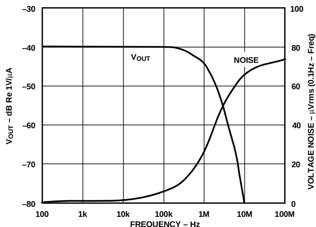
Figure 49. Total Integrated Voltage Noise & V_{OUT} of Amorphous Detector Preamplifier
