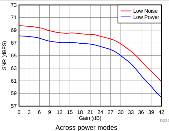
Figure 34. Signal-to-Noise Ratio vs Gain
