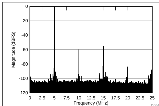
Figure 105. FFT for VCNTL = 0 V
