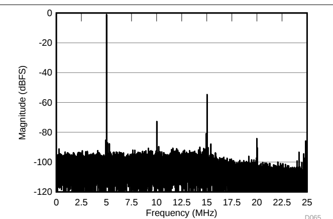
Figure 106. FFT for VCNTL = 0.9 V
