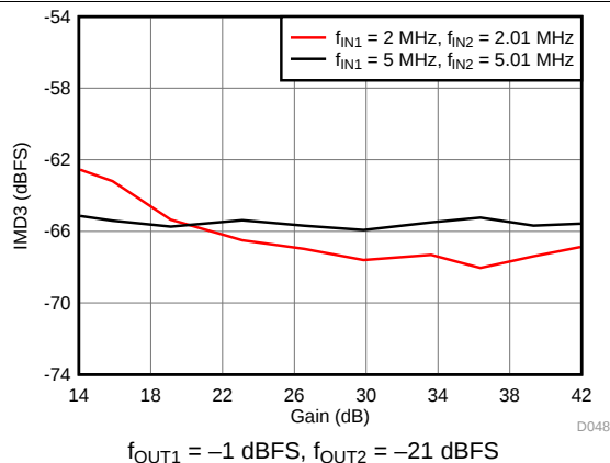
Figure 48. IMD3 vs Gain
