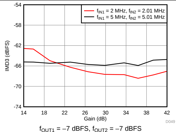
Figure 49. IMD3 vs Gain
