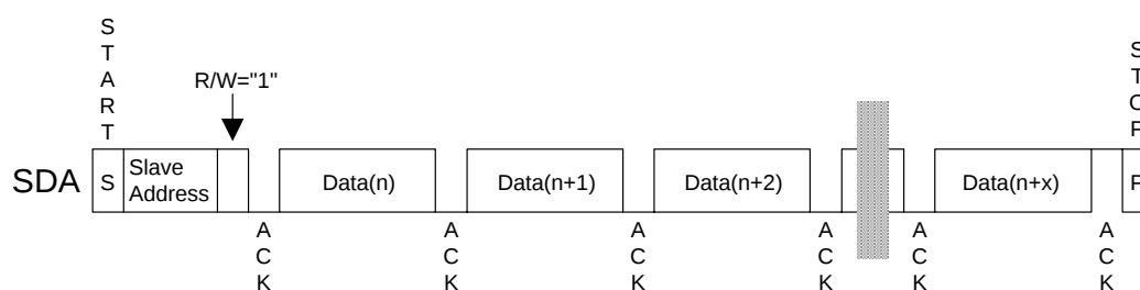
Figure 68. CURRENT ADDRESS READ
