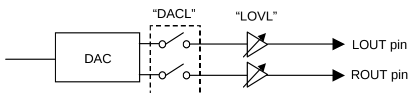
Figure 45. Stereo Line Output
