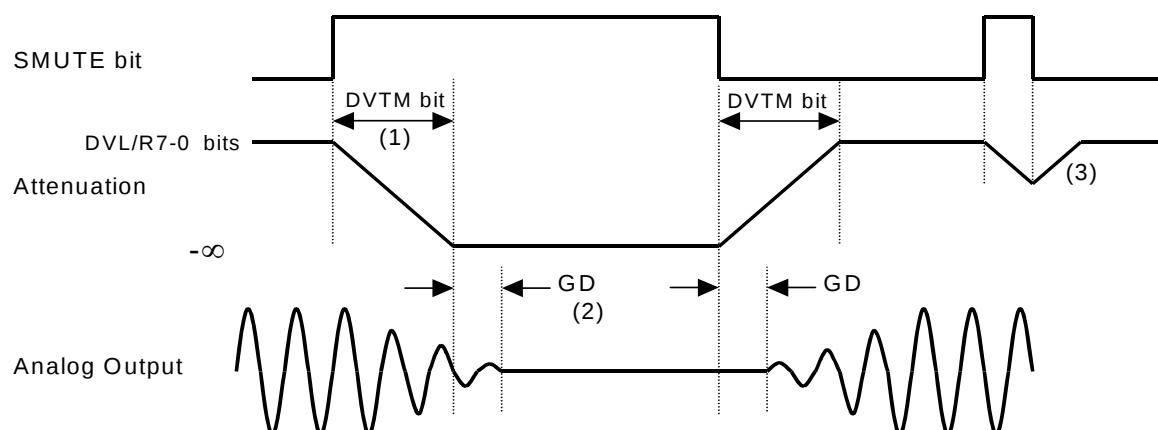
Figure 39. Soft Mute Function
