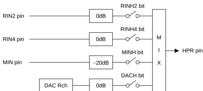
Figure 60. HPR Mixing Circuit (AIN3 bit = "0", HPG bit = "0")
