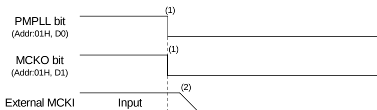
Figure 85. Clock Stopping Sequence (3)
