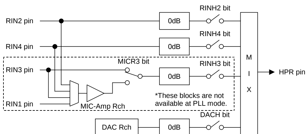
Figure 62. HPR Mixing Circuit (AIN3 bit = "1", HPG bit = "0")
