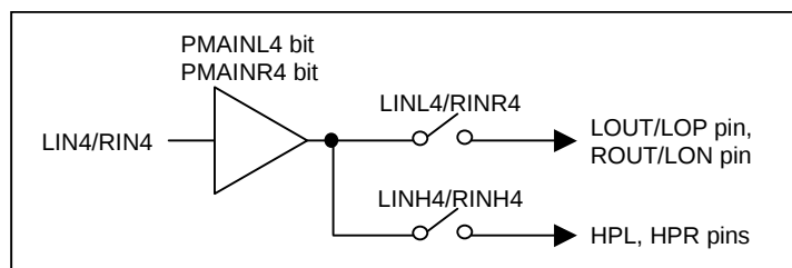
Figure 42. Analog Mixing Circuit (LIN4/RIN4)
