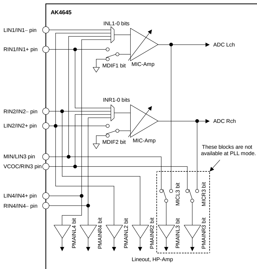
Figure 32. Mic/Line Input Selector
