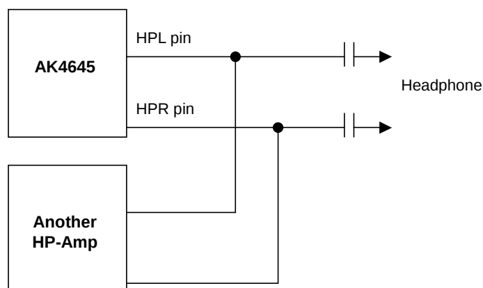
Figure 58. Wired OR with External HP-Amp
