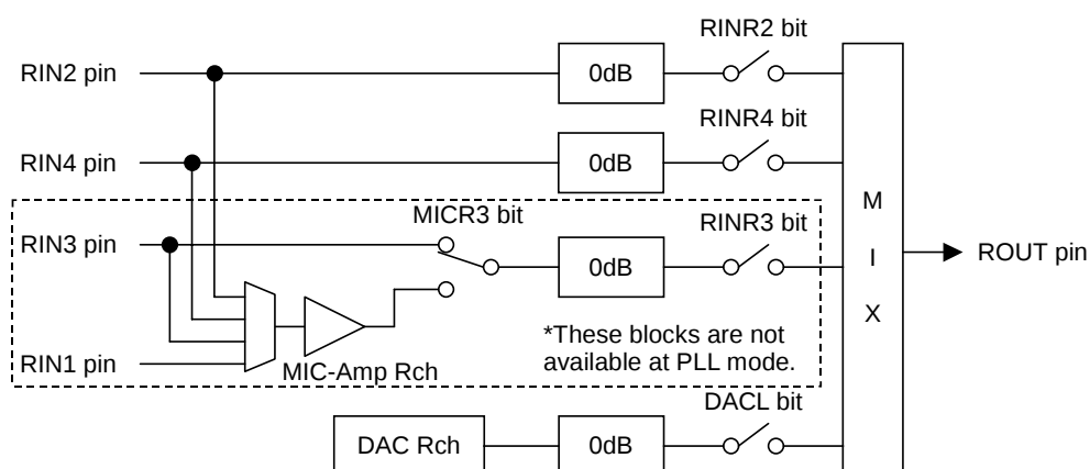
Figure 51. ROUT Mixing Circuit (AIN3 bit = "1", LOVL bit = "0")
