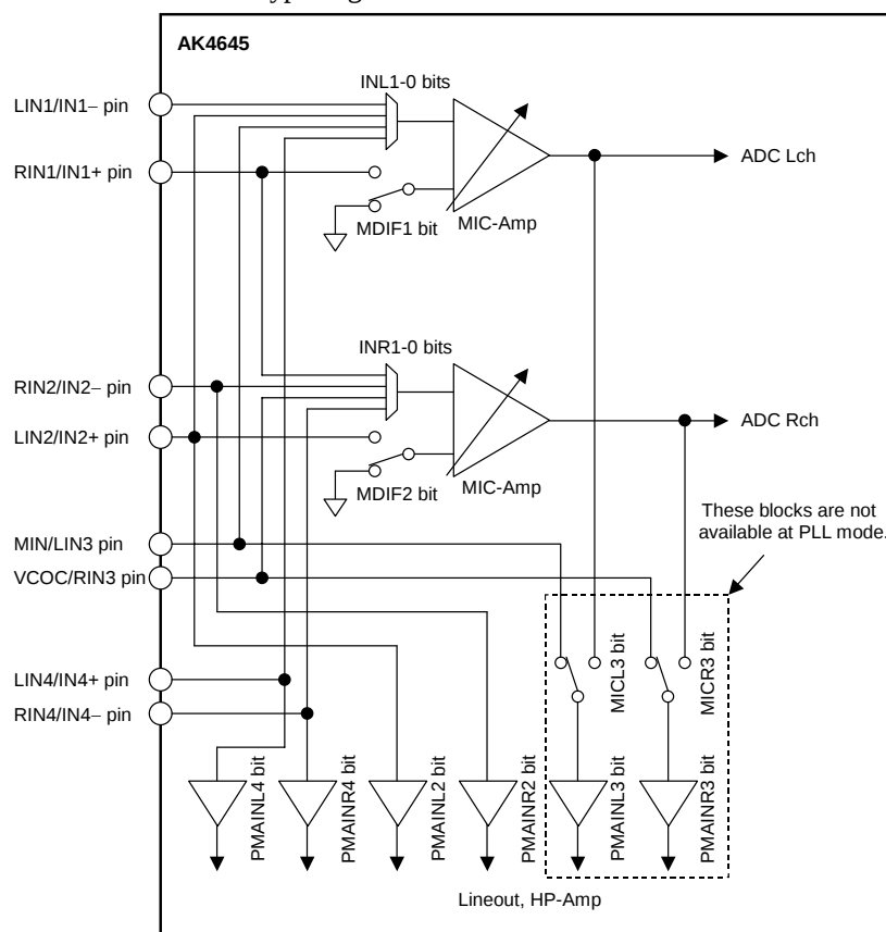
Figure 40. Analog Mixing Circuit (Stereo Input)
