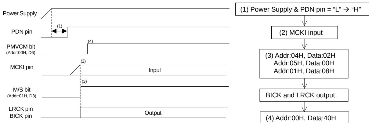
Figure 79. Clock Set Up Sequence (5)
