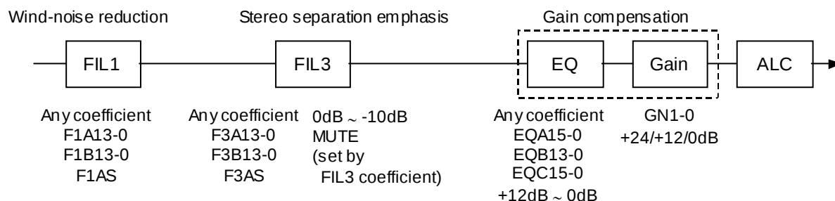
Figure 35. Digital EQ/HPF/LPF
