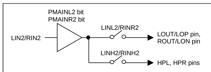
Figure 41. Analog Mixing Circuit (LIN2/RIN2)
