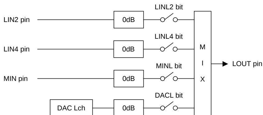
Figure 48. LOUT Mixing Circuit (AIN3 bit = "0", LOVL bit = "0")
