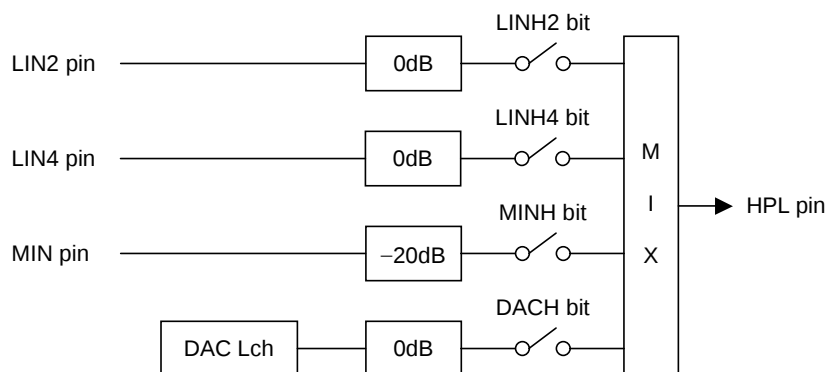
Figure 59. HPL Mixing Circuit (AIN3 bit = "0", HPG bit = "0")
