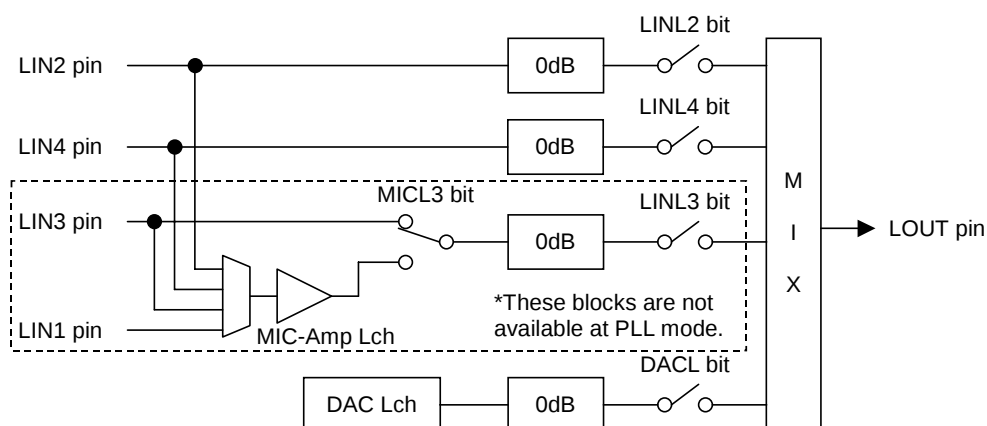
Figure 50. LOUT Mixing Circuit (AIN3 bit = "1", LOVL bit = "0")
