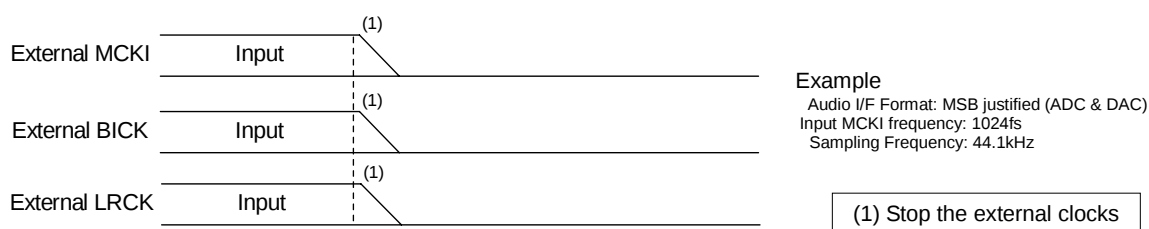
Figure 86. Clock Stopping Sequence (4)
