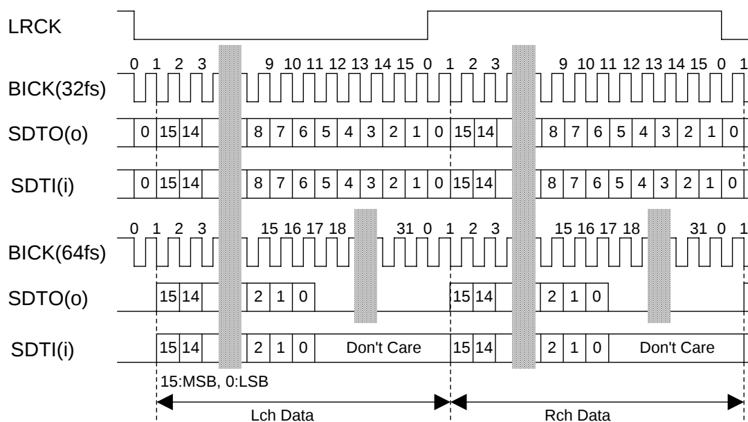
Figure 31. Mode 3 Timing
