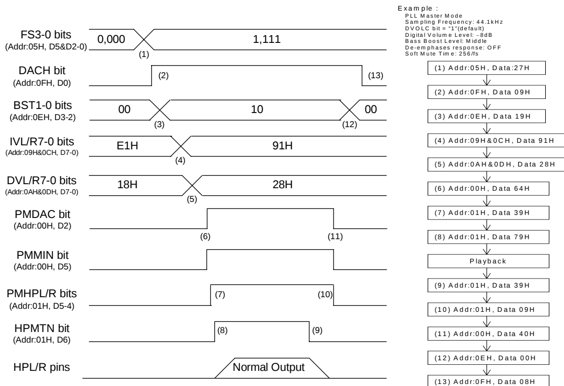
Figure 81. Headphone-Amp Output Sequence
