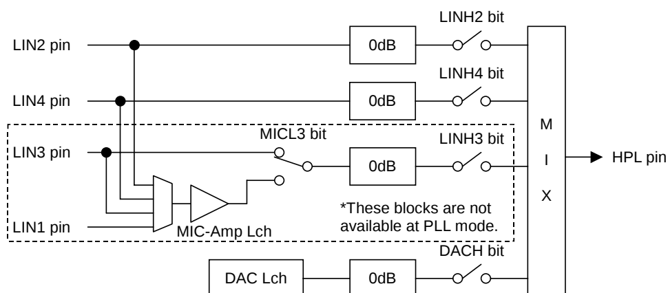
Figure 61. HPL Mixing Circuit (AIN3 bit = "1", HPG bit = "0")
