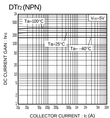
Fig.5 DC current gain vs. Output current characteristics
