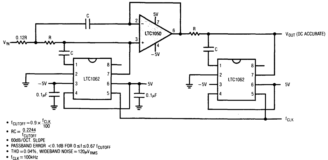
DC Accurate 10th Order Max Flat Lowpass Filter
