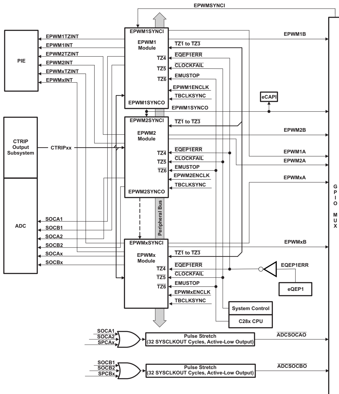
Figure 6-37. ePWM
