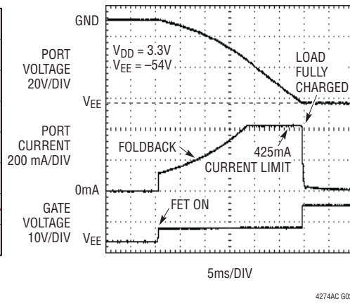
Powering Up into a 180 \mu F Load
