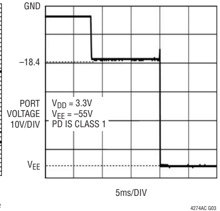
802.3af Classification in AUTO Pin Mode
