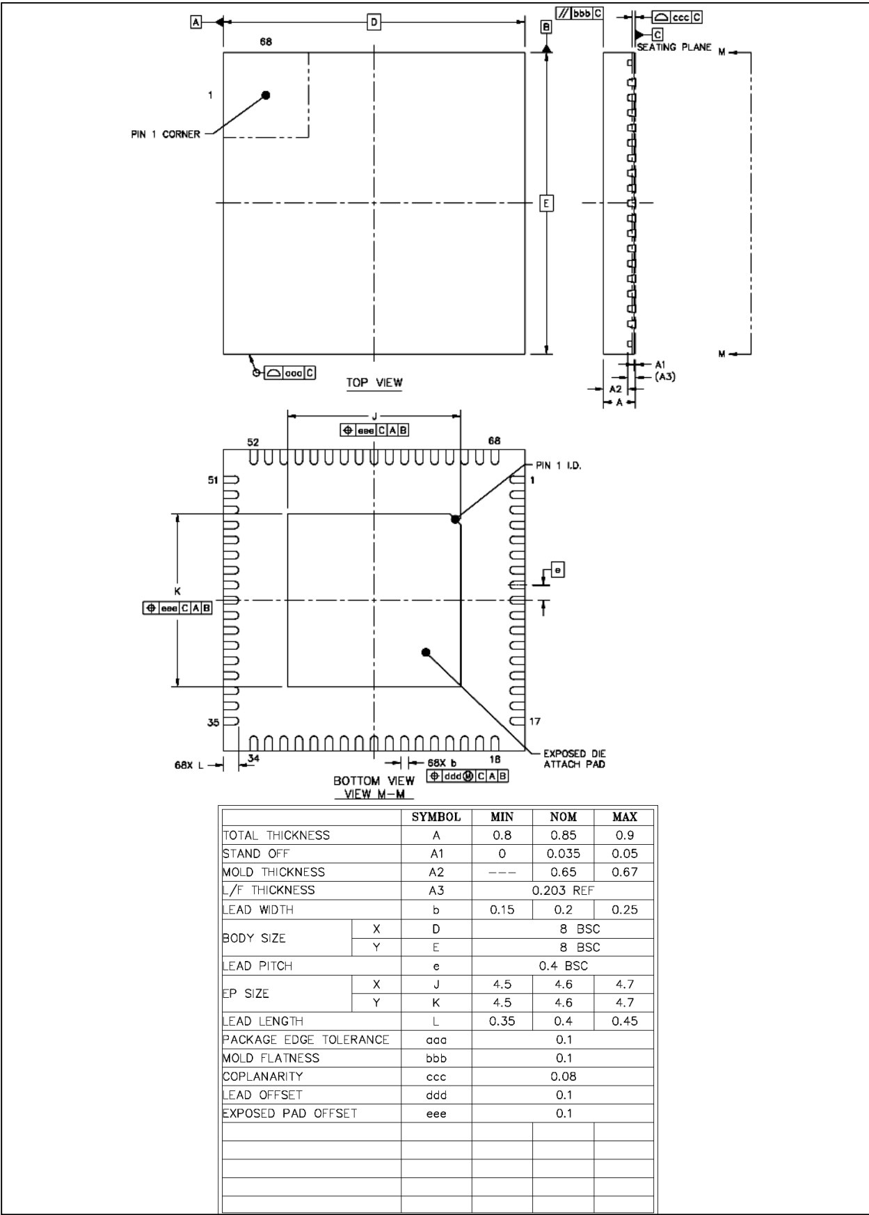
QFN68 8x8 Chip Outline (IS2025S)
