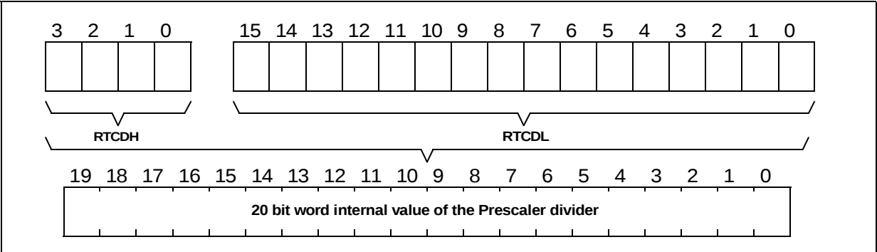
Figure 53 : DIVIDER Counters
