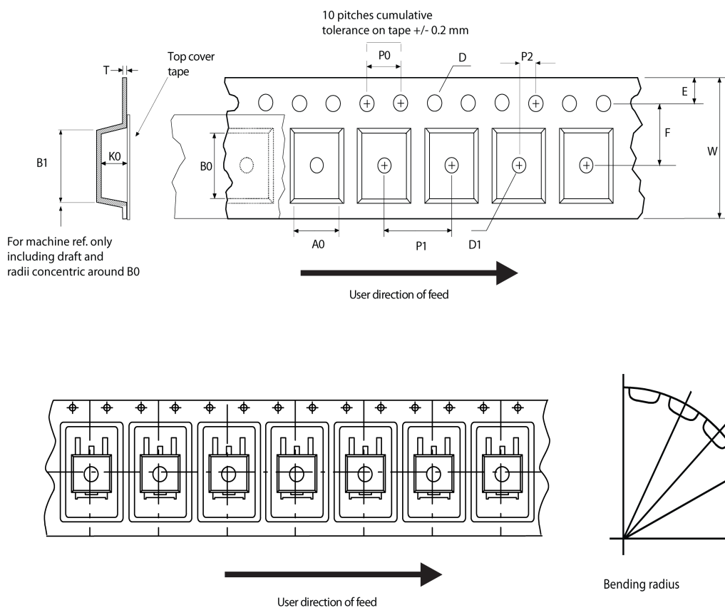
Figure 28. Tape outline
