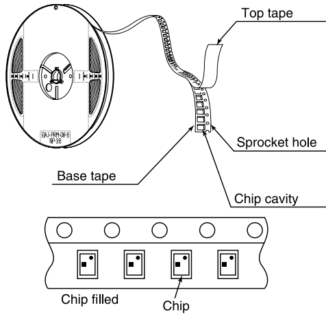
Embossed Tape
