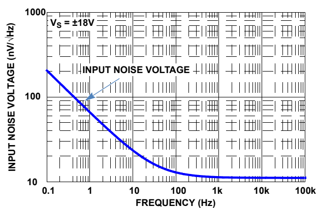
FIGURE 49. SIMULATED INPUT NOISE VOLTAGE
